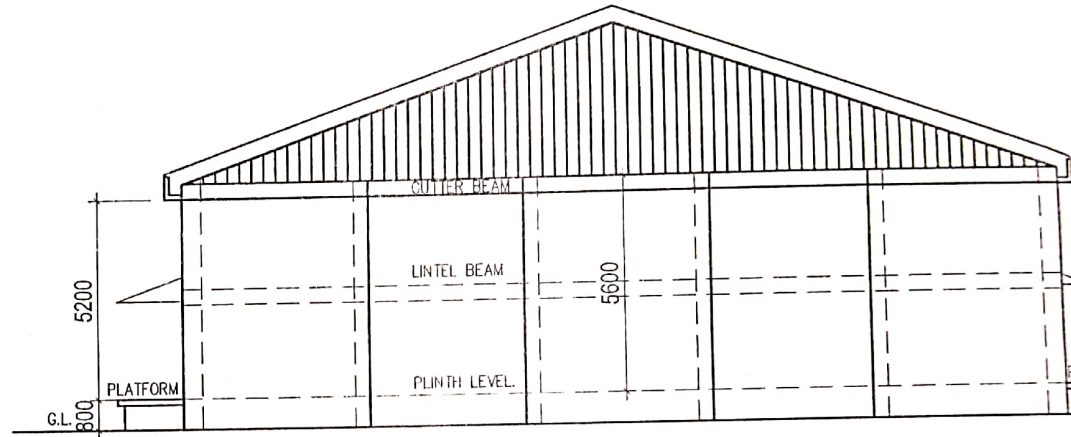
ELEVATION - B & D
