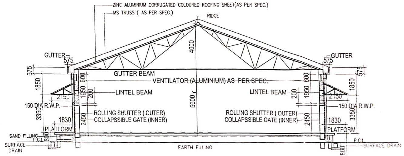
CROSS SECTION-AA
